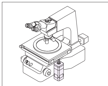
Vertical fine-tuning of table position
